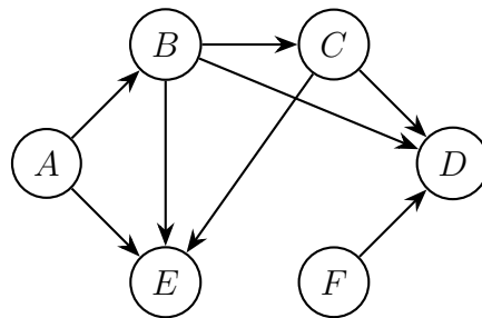
Figure 1: Directed G for topological sort.
